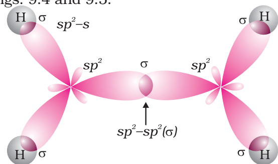
Fig. 9.4 Orbital picture of ethene depicting \sigma bonds only
