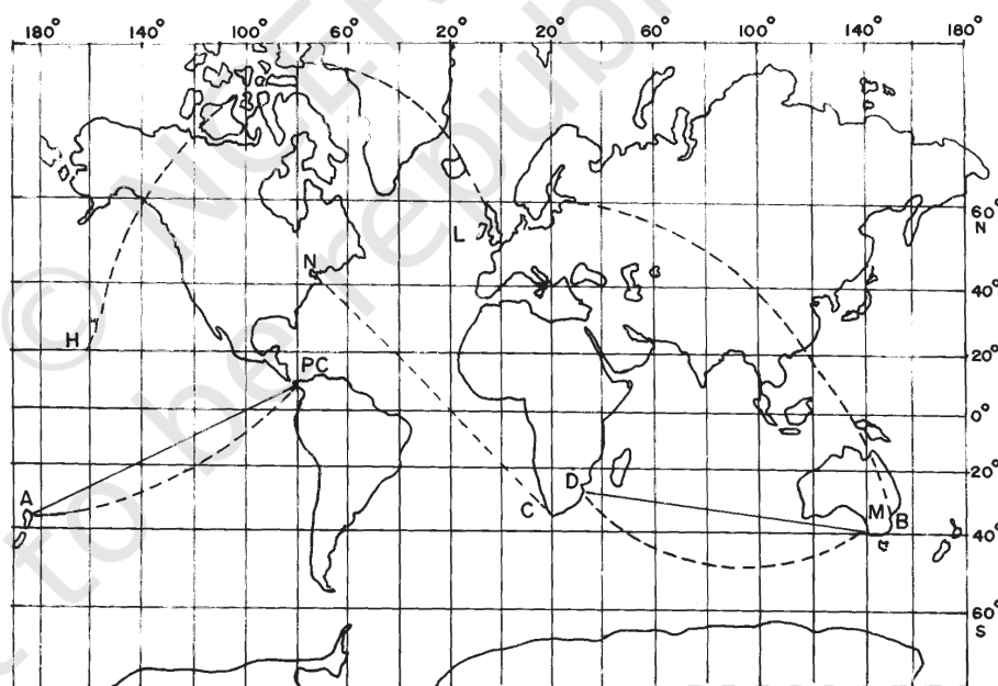
Figure 4.6 Straight lines are Laxodromes or Rhumb lines and Dotted lines are great circles
